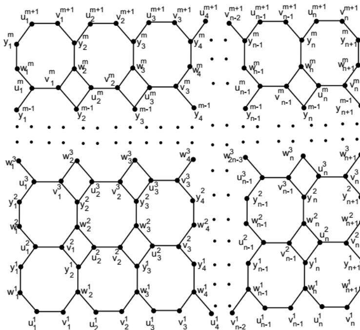
FIGURE 1. The Octagonal grid O_n^m .
